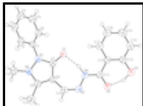
Fig. 1. The molecular structure of the title compound, with 50% displacement ellipsoids. The hydrogen bonds are shown with dashed lines.
